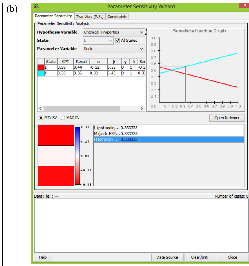
Fig. 5. Parameter sensitivity analysis function graph, for the hypothesis variable chemical properties node, using the parameter variable sodic and saline (block b). Sensitivity values are shown in the network diagram (block a).
