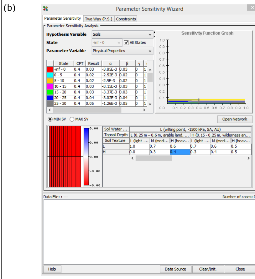
Fig. 1. Parameter sensitivity analysis function graph, for the hypothesis variable soils node, using the parameter variable physical properties (block b). As the hypothesis node has many states the graph shows many overlapping function lines. Sensitivity values are shown in the network diagram (block a).
