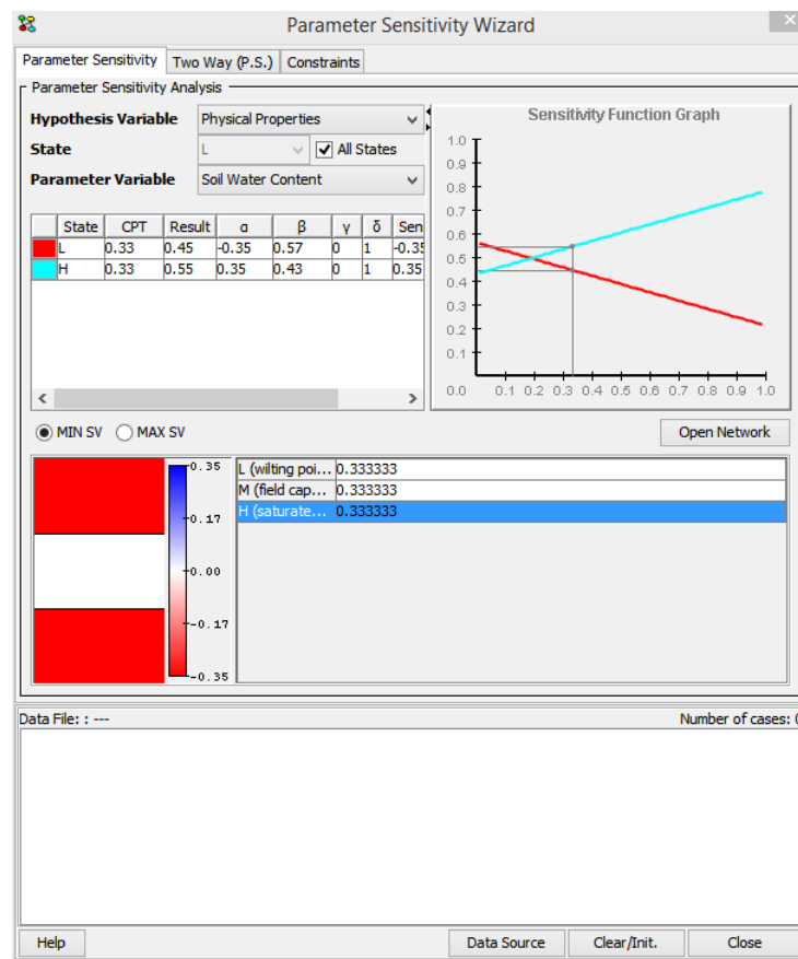
Fig. 2. Parameter sensitivity analysis function graph, for the hypothesis variable physical properties node, using the parameter variable soil water content (block b). Sensitivity values are shown in the network diagram (block a).
